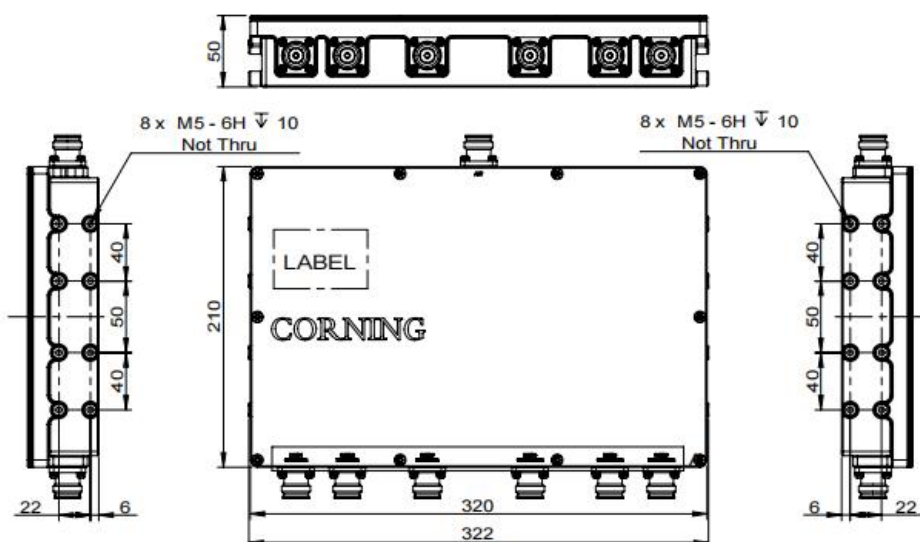
Figure 89.dHRU-G2-COMB-L combiner
