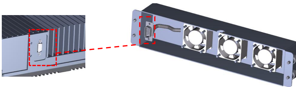
Figure 78. Fan Connection with DB15
