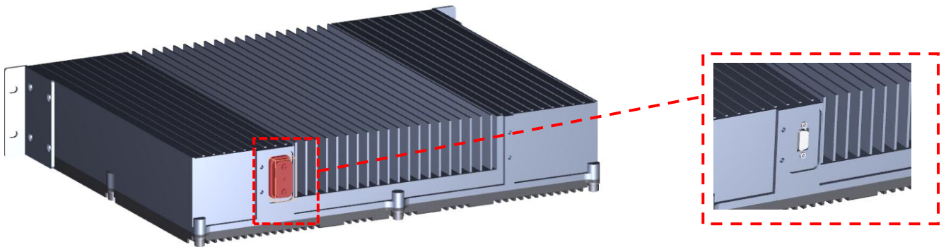
Figure 77. Fan Connection
