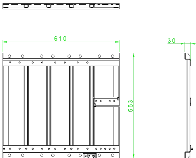
Figure 81.dMRU bracket dimensions
