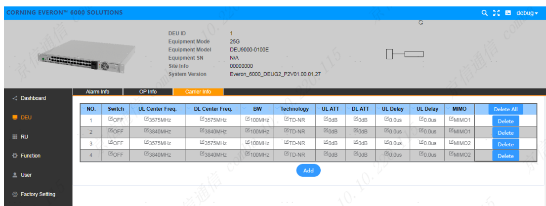
Figure 6.3-4 dLRU channel 3 SISO carrier configuration page
