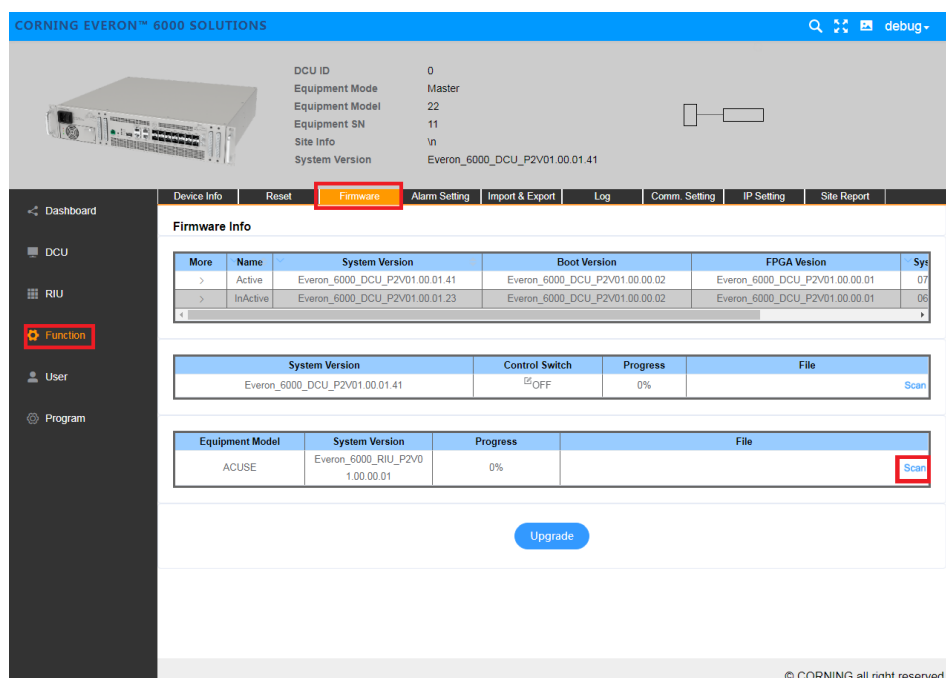
Figure 5.1-2 WEB OMT login interface
