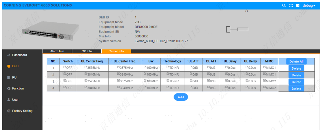
Figure 6.3-5 dLRU channel 2 MIMO carrier configuration page
