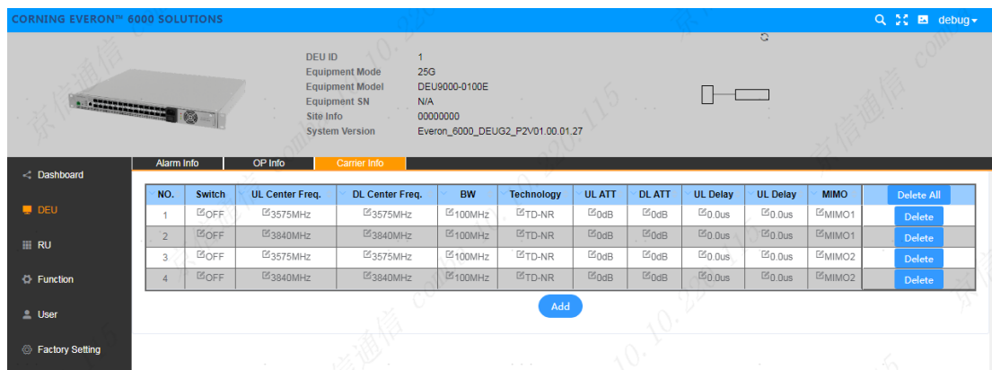
Figure 6.3-6 dLRU channel 4 MIMO carrier configuration page
