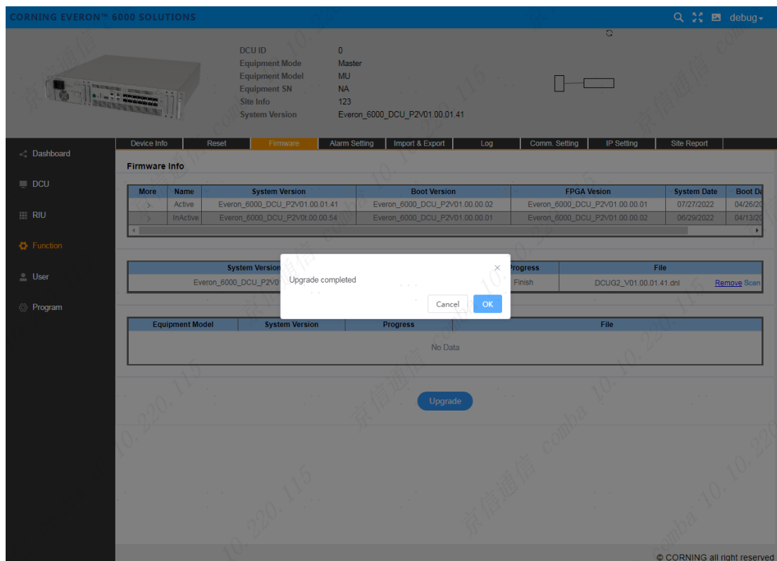
Figure 5.2-3 DCU software upgrade package upload completed
