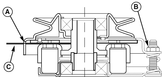
Figure 27. Adjust PTO Clutch
