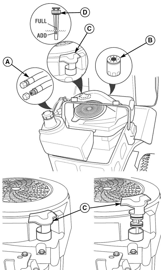
Figure 29. Oil Change
