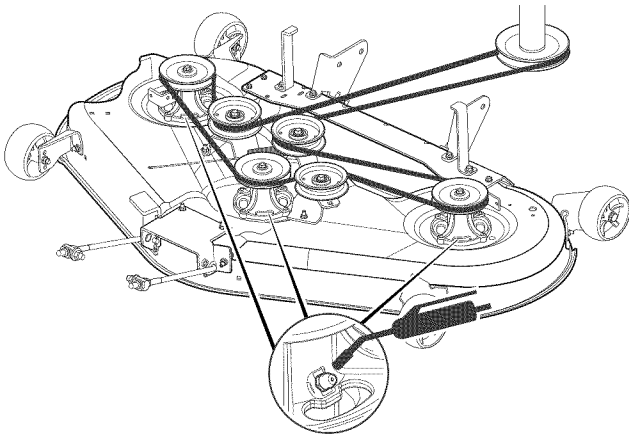
Figure 18. Mower Lubrication
