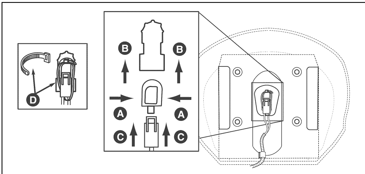
Figure 2. Installing the Seat Safety Switch
