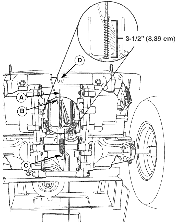
Figure 34. Brake Adjustment
