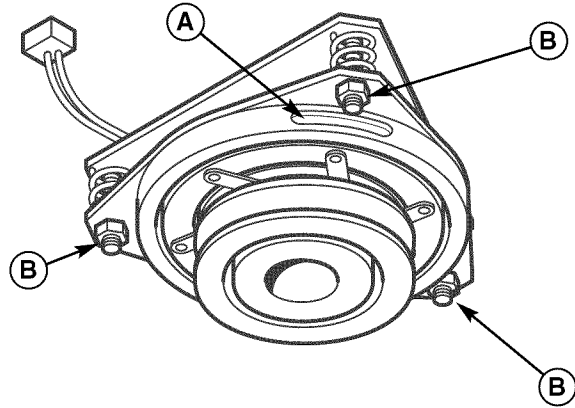
Figure 26. PTO Clutch Adjustment
