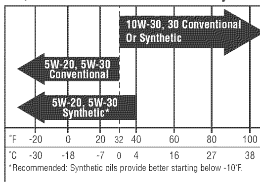
Figure 28. Recommended Engine Oil
