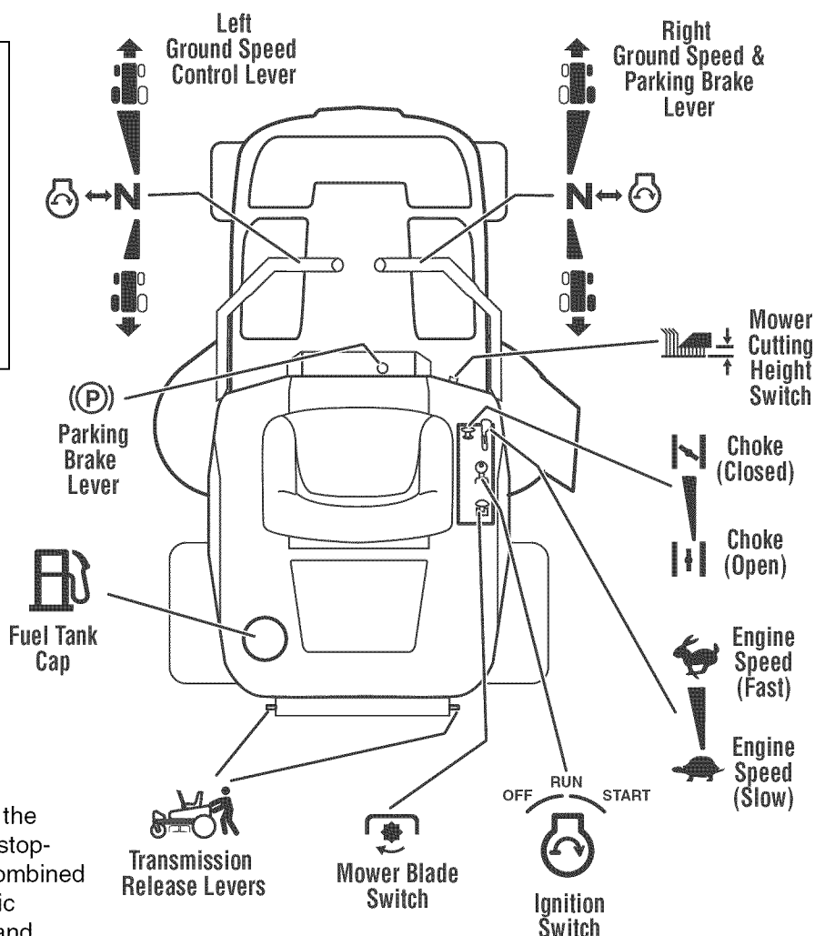
Figure 4. Controls
