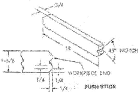
NOTE: All dimensions in inches
