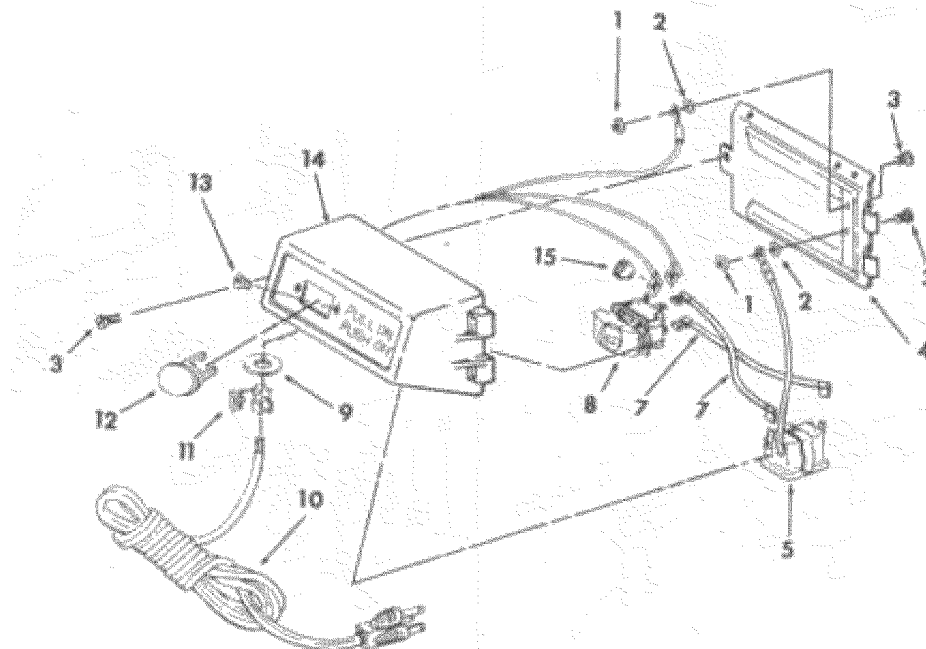
FIGURE 6 – 62592 SWITCH BOX ASSEMBLY
