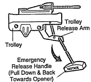
Lockout position
