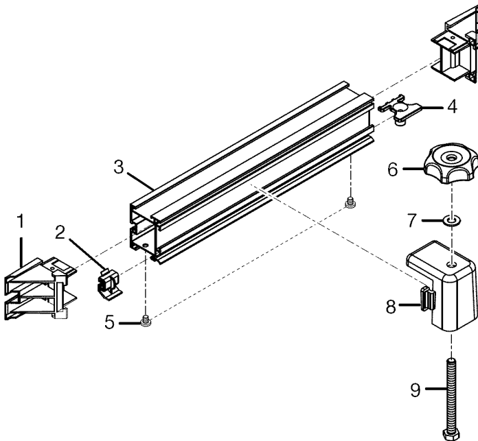
FIGURE B: MITER FENCE
