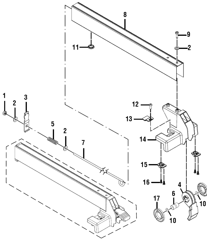
FIGURE C: RIP FENCE
