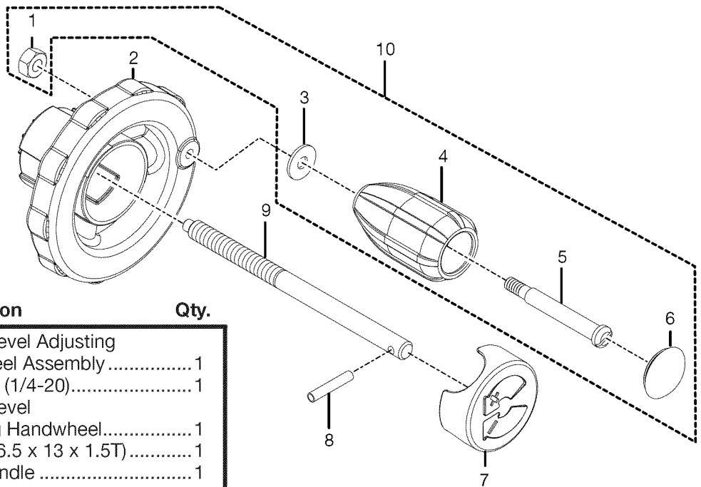
FIGURE D: HEIGHT ADJUSTING HANDWHEEL
