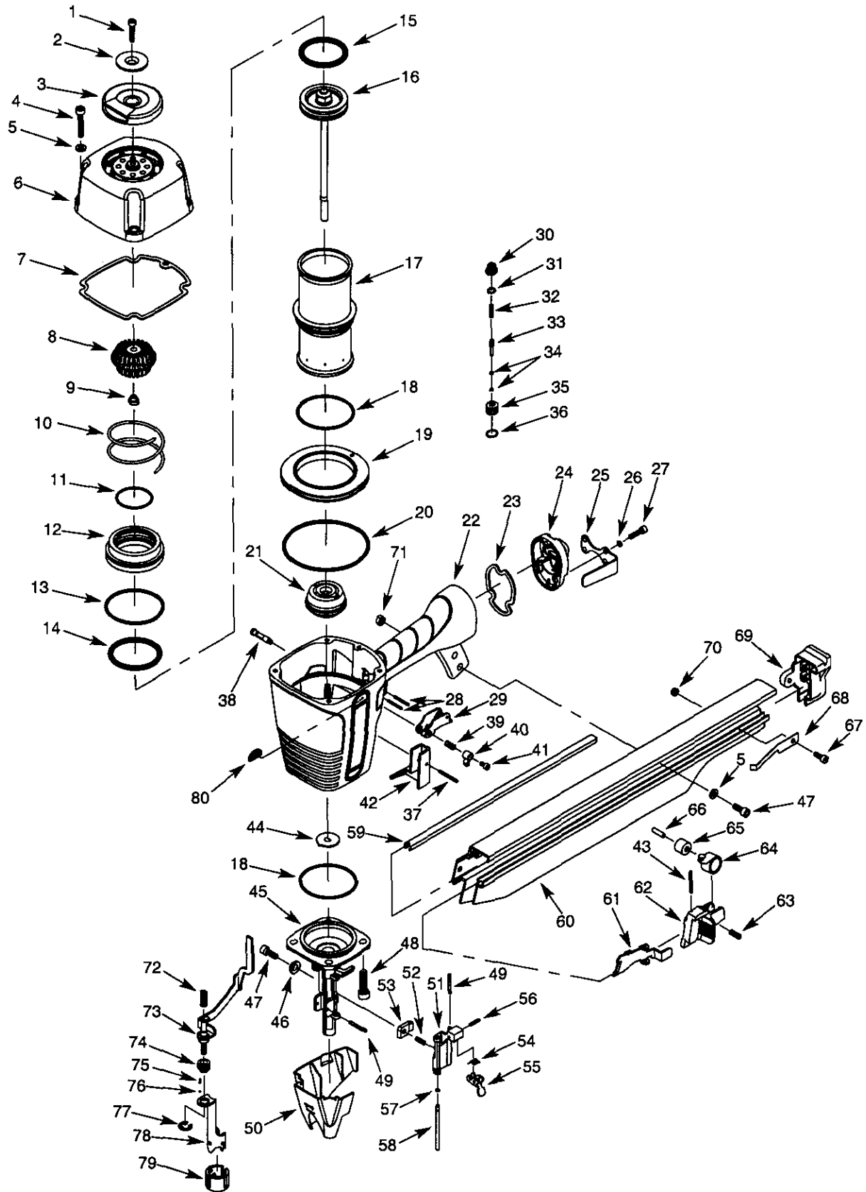
Figure 12 - Replacement Parts Illustration For Framing Nailer
