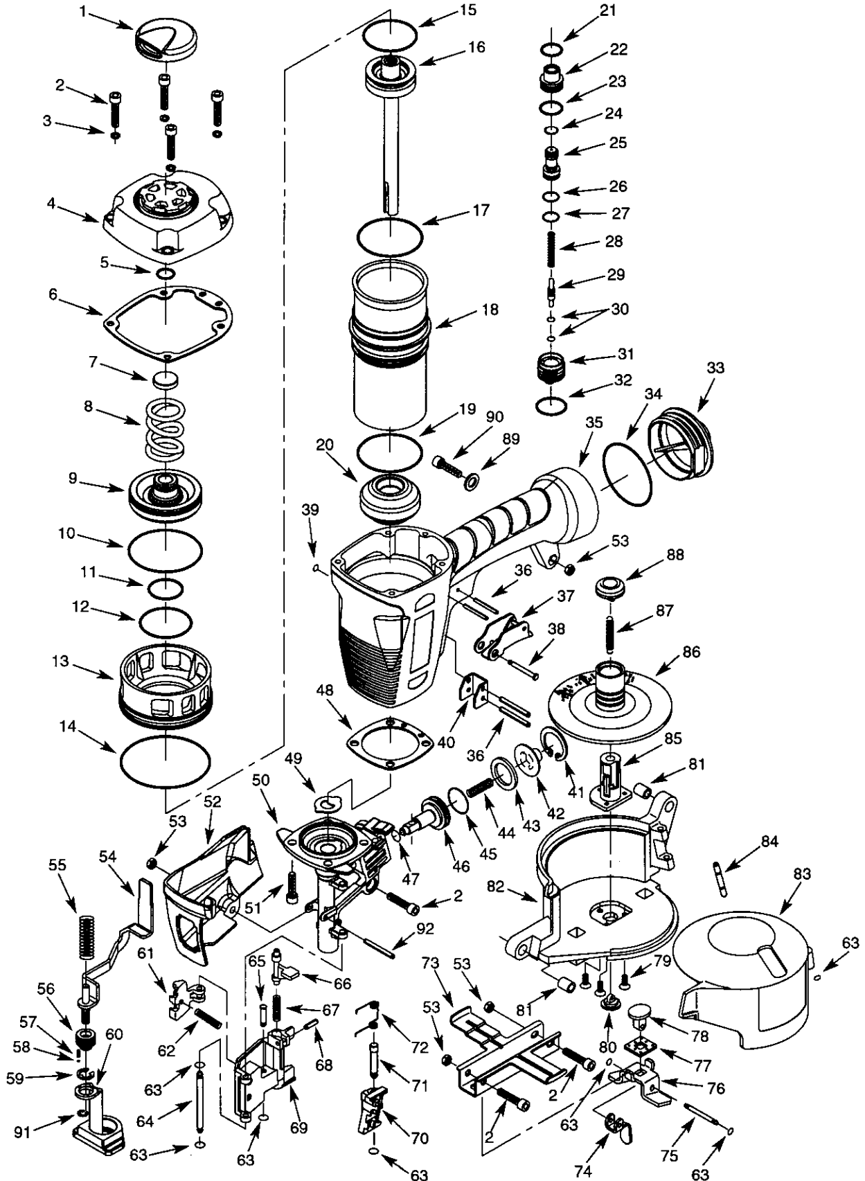
Figure 10 - Replacement Parts Illustration For Nailers
