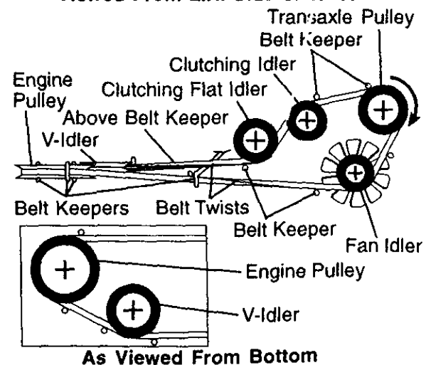
Tractor V-Belt Drive Schematic Viewed From L.H. Side of Tractor
