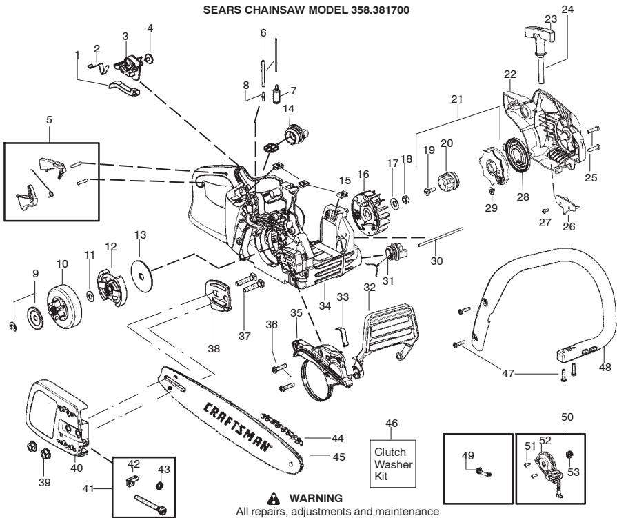
SEARS CHAINSAW MODEL 358.381700
