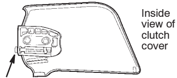
Adjustment located on clutch cover
