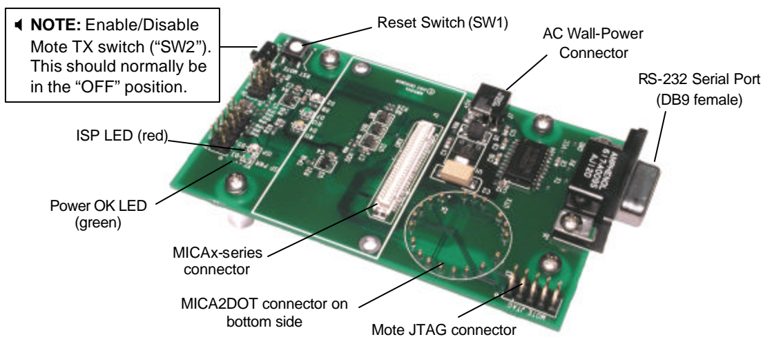
Fig 6.1 Photo of top view of an MIB510CA.
