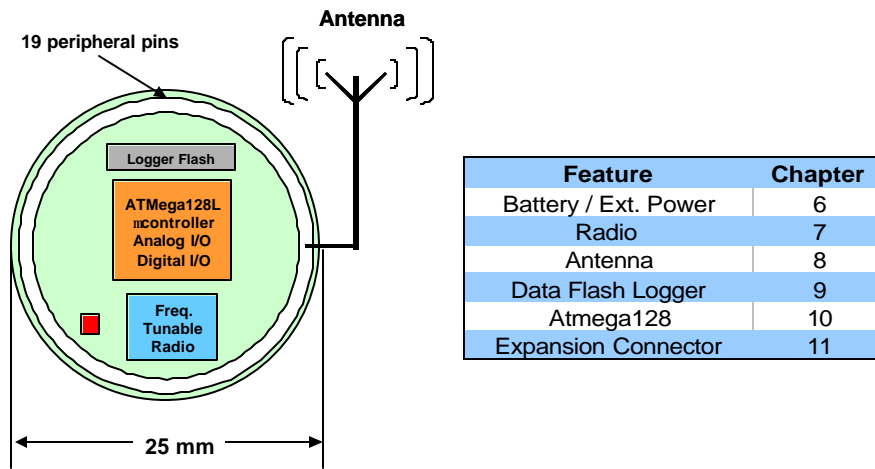
Figure 4-1. Block diagram of the MICA2DOT and listing of Chapters that discuss the components in greater detail.
