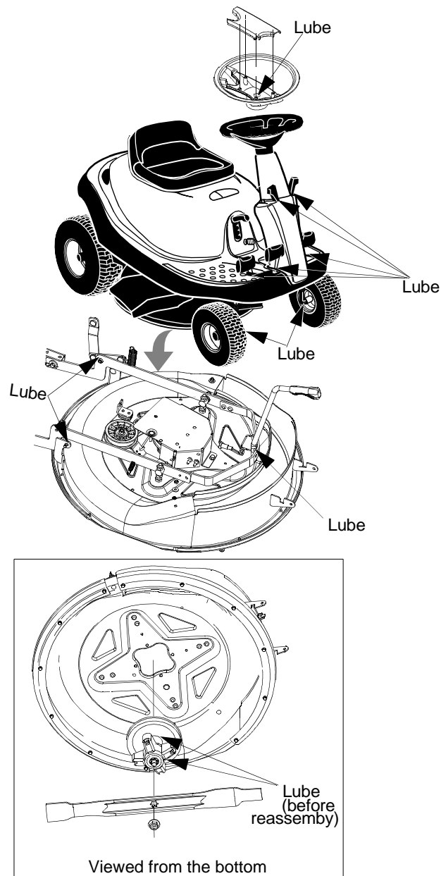
Figure 19: Lubrication Chart
