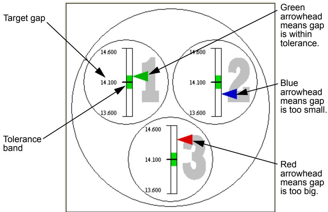
Figure 3.6: Graphical Readouts
