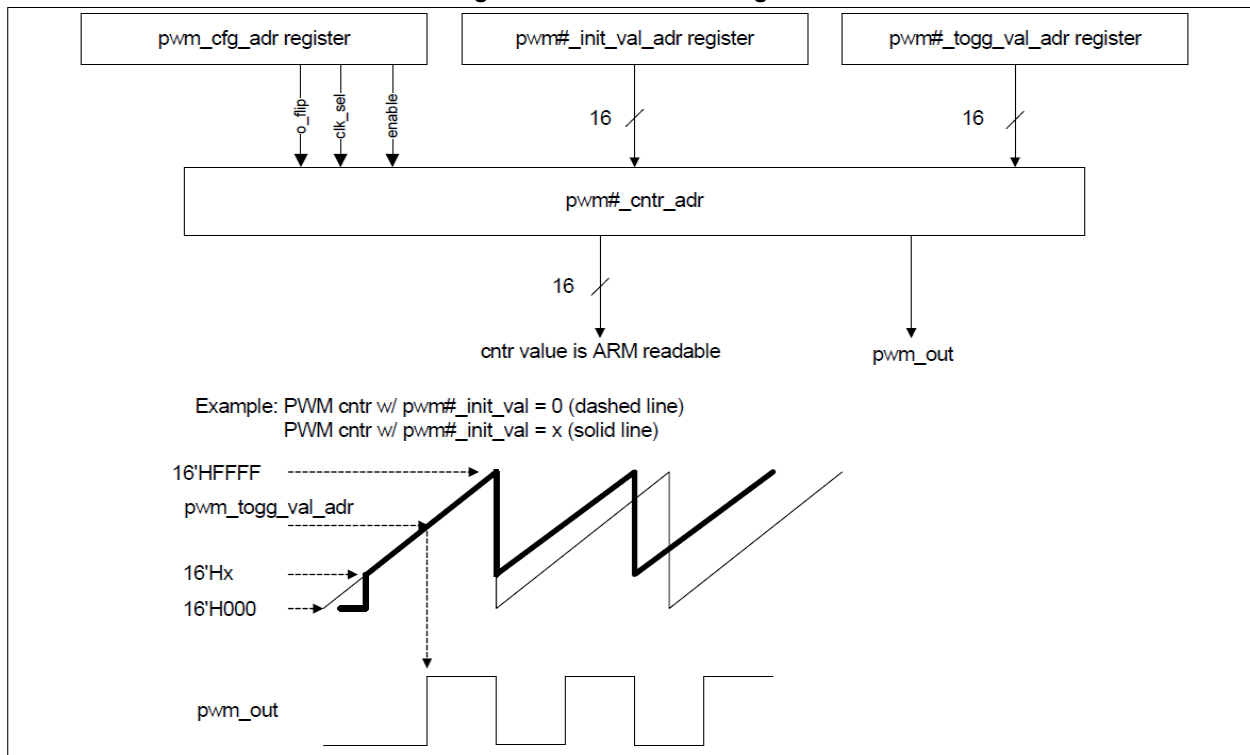
Figure 12. PWM Block Diagram
