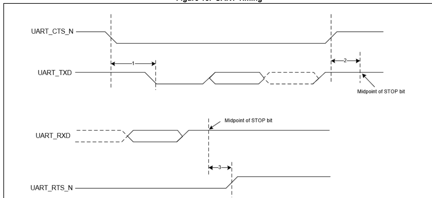
Figure 13. UART Timing
