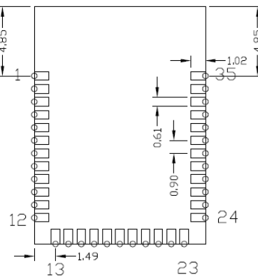
Figure 3. Solder Pad Dimensions (Seen from Bottom)
