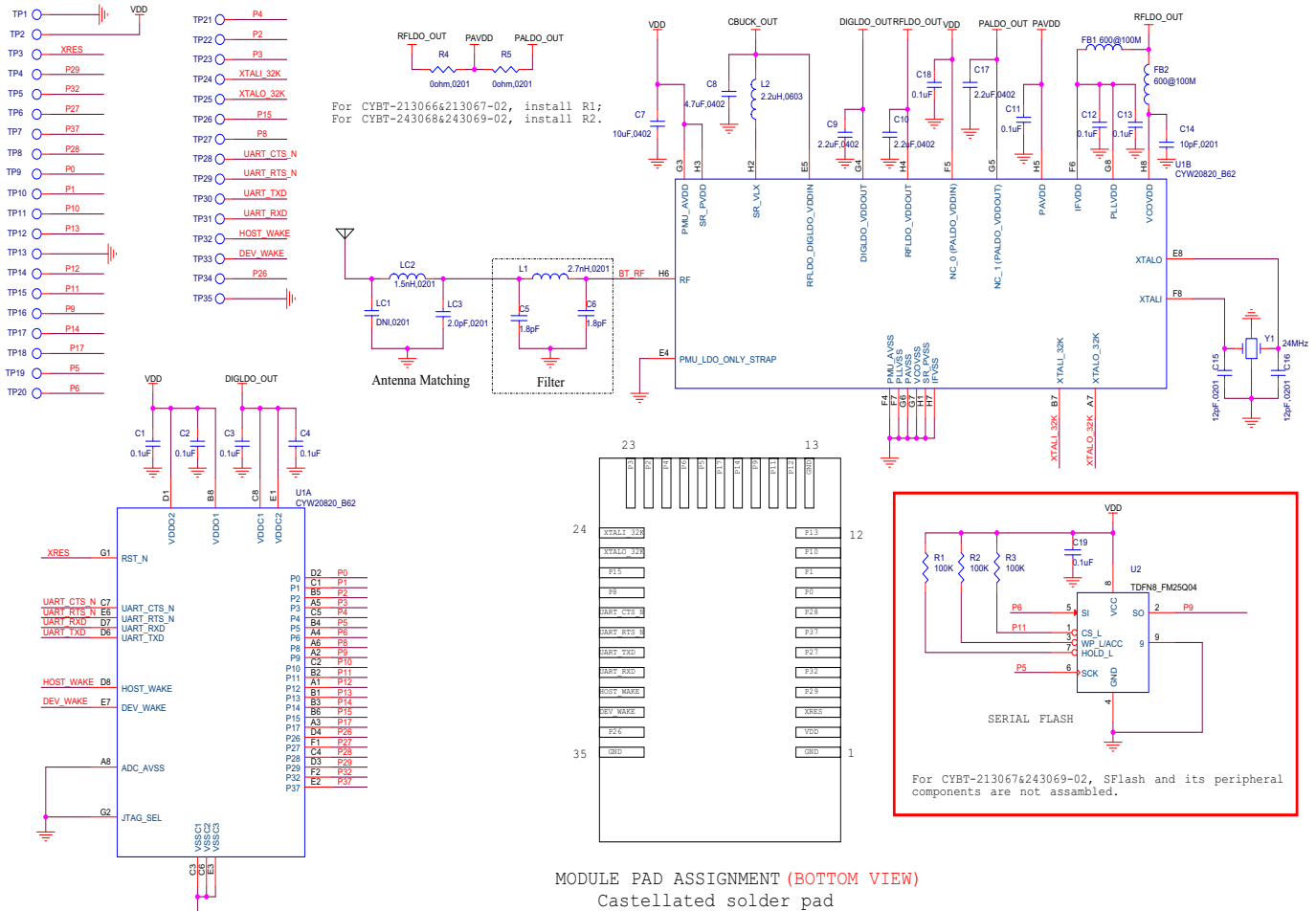
Figure 8. CYBT-213066-02/CYBT-213067-02 Schematic Diagram
