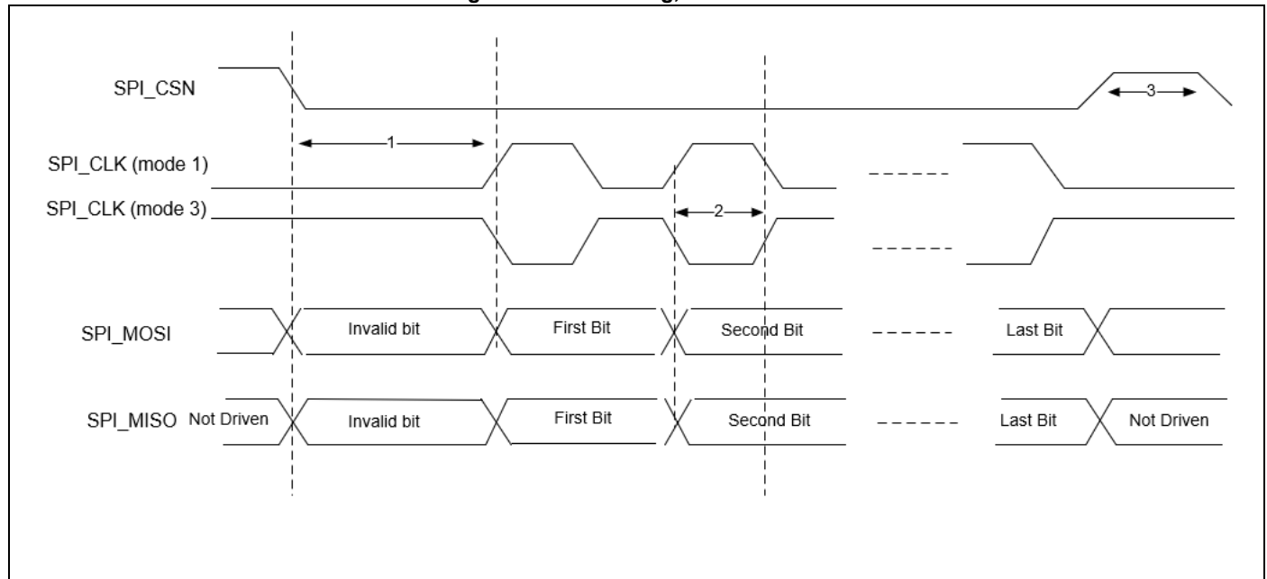
Figure 15. SPI Timing, Mode 1 and 3
