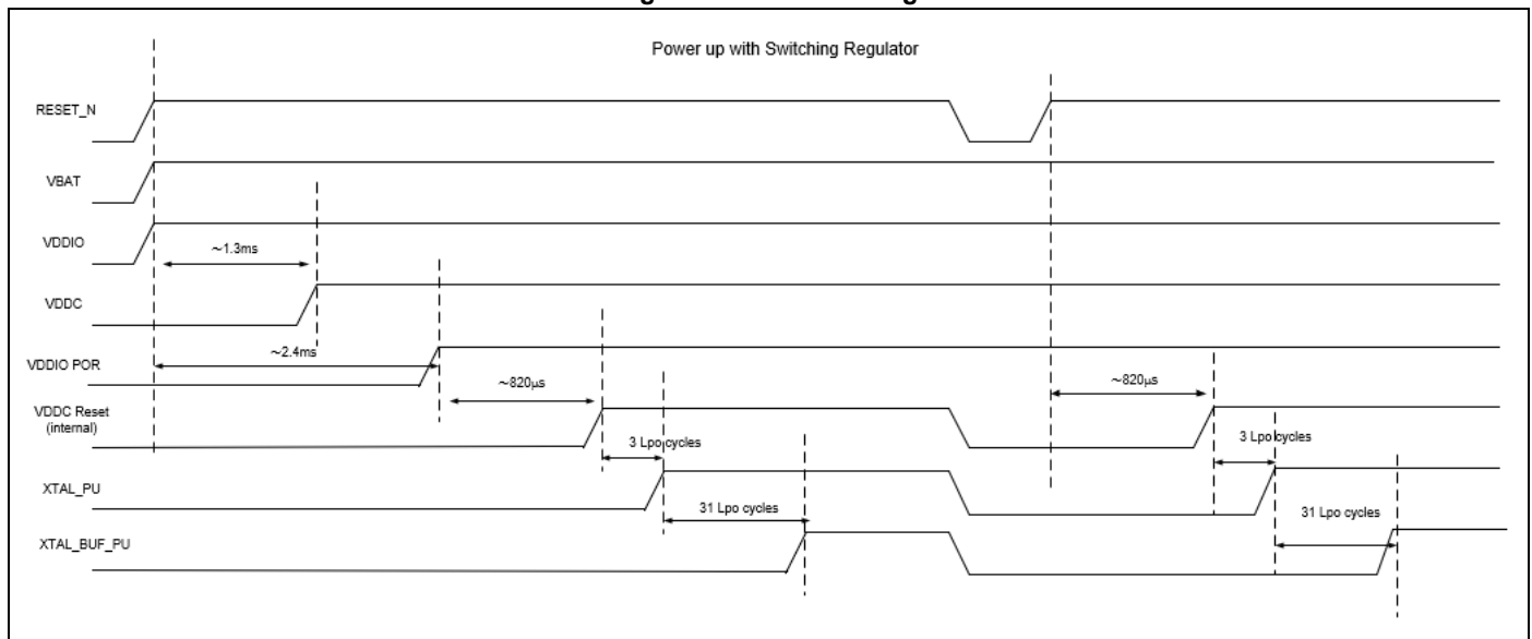
Figure 10. Reset Timing
