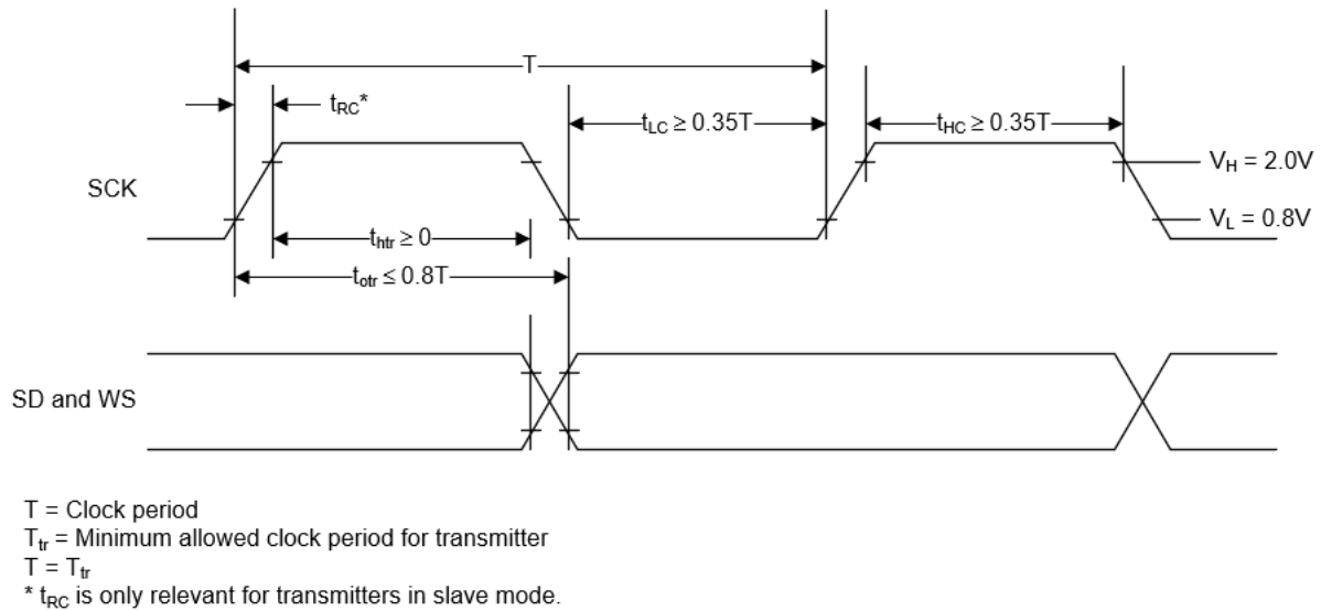
Figure 17. I 2 S Transmitter Timing
