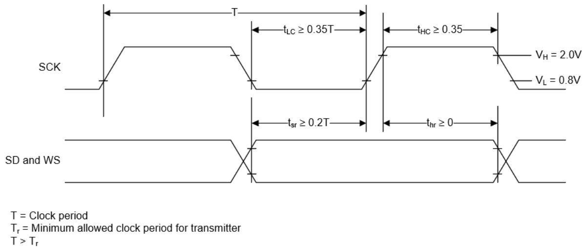
Figure 18. I 2 S Receiver Timing
