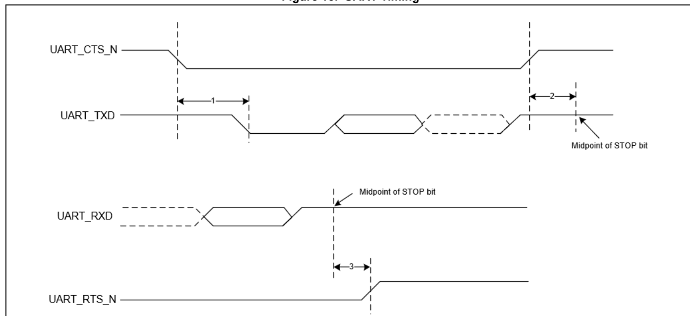
Figure 13. UART Timing
