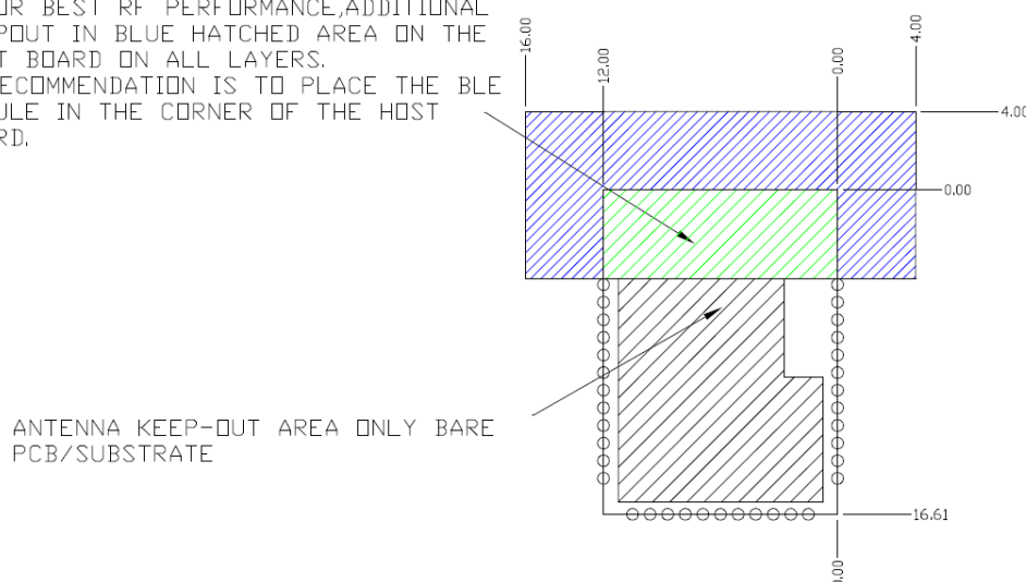
Figure 4. Optional Additional Host PCB Keep Out Area Around the CYBT-213066-02/CYBT-213067-02 PCB Antenna
