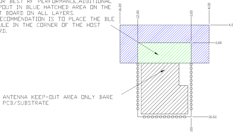
Figure 4. Optional Additional Host PCB Keep Out Area Around the CYBT-243068-02/CYBT-243069-02 PCB Antenna
