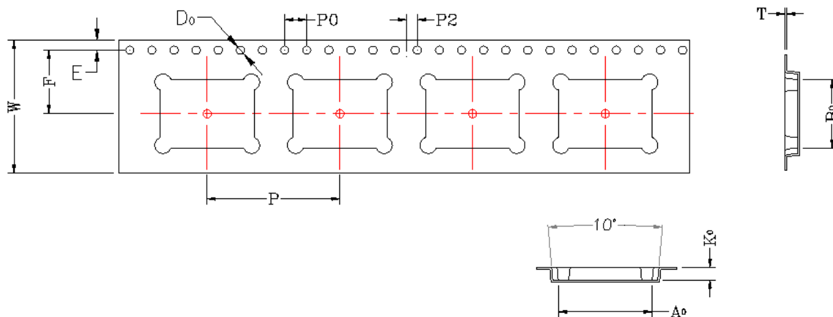
Figure 20. Component Orientation in Tape and Unreeling Direction
