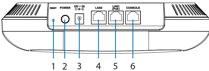
Figure 2: Rear Connectors
