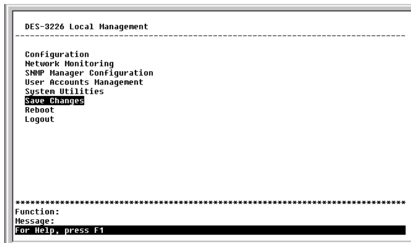
Figure 6-5. Main menu
