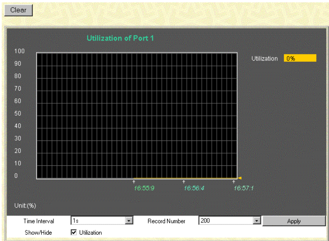
Figure 7-36. Utilization window
