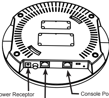
Figure 2. DWL-6610AP Rear Panel
