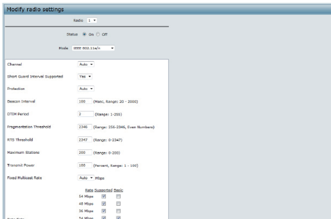
Figure 20 - Modify Radio Settings
