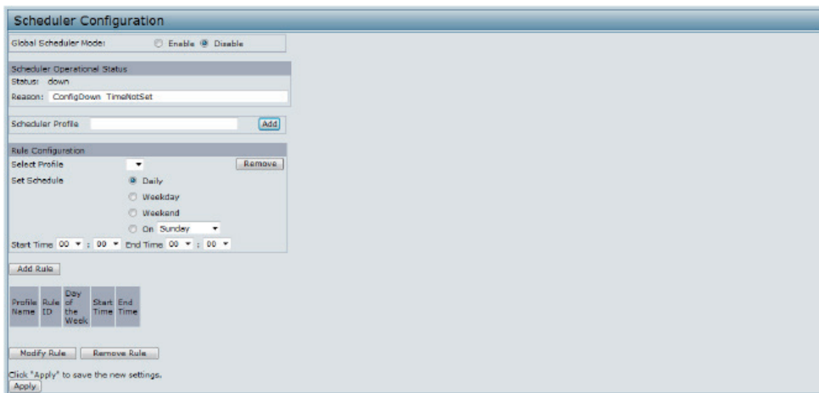
Figure 21 - Scheduler Configuration
