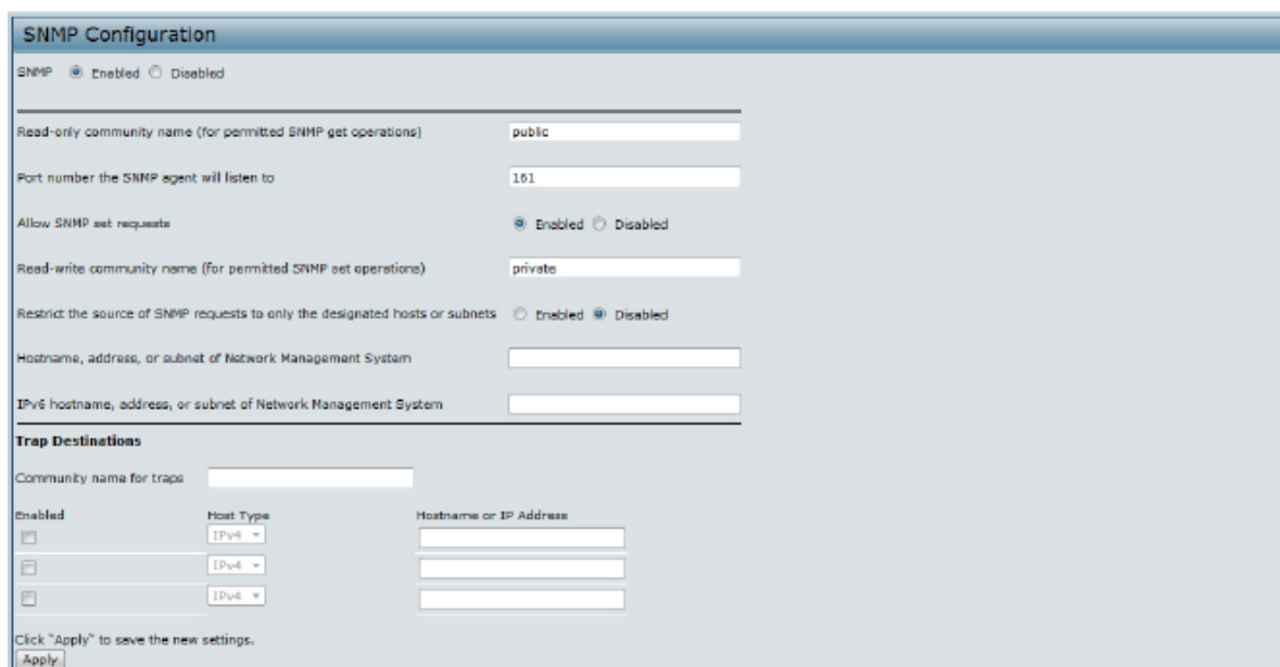
Figure 37 - SNMP Configuration
