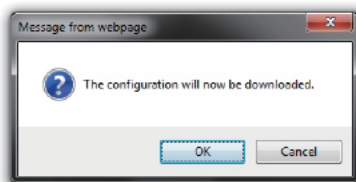
Figure 50 - Confirmation Prompt
