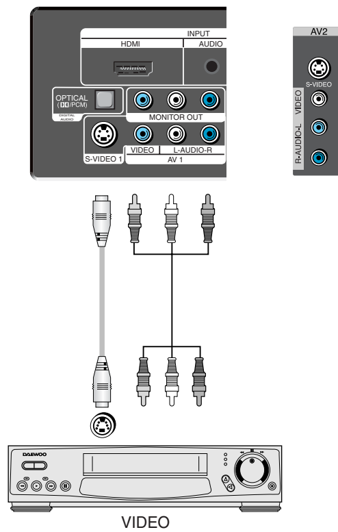
REAR AND SIDE OF THE TV SET
