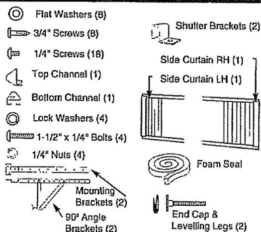
Fig. 1 Installation Hardware
