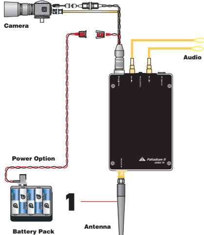
Typical Wiring Configuration
