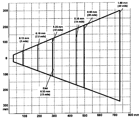
Reading Zones (10° skew angle)
