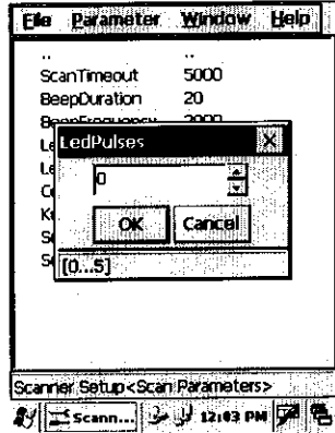
Selecting Data Capture Setup Parameters
