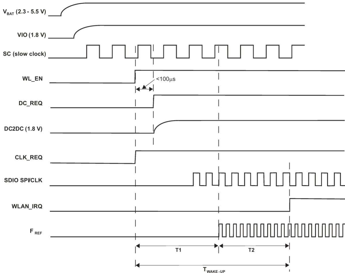
Figure 2 Power-up Sequence Requirements
