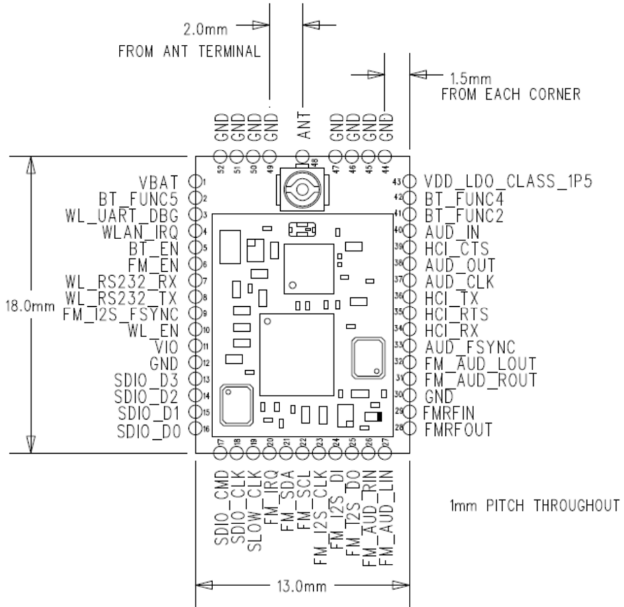
Figure 1 Pinout (Top View)
