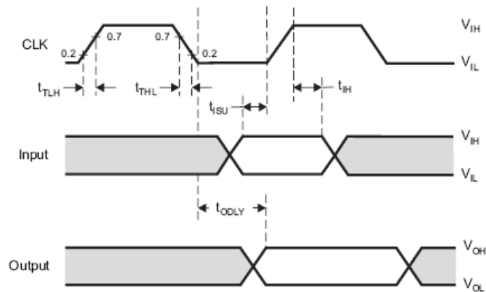
Figure 10 SDIO Clock Timing
