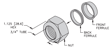
FSV-SS 3/4 TS-NPT (A9306)
