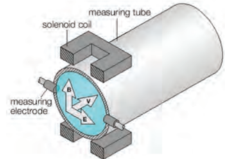
FCMI monitors utilize Faraday's magnetic inductive principle
