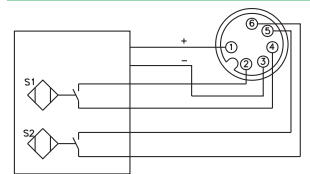
Mating Cordset: RKC 6T-*
