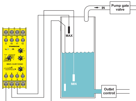
Example Application using MK91-12-R/...
