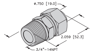
FSV-SS 3/4 TS-NPT (A9306)
