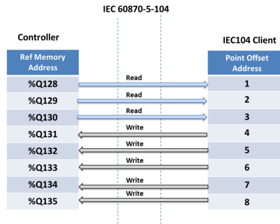
Figure 18: Read/Write Interaction between Controller and IEC104 Client (Case 2)
