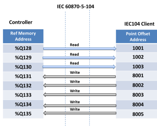
Figure 16: Read/Write Interaction between Controller and IEC104 Client (Case 1)
