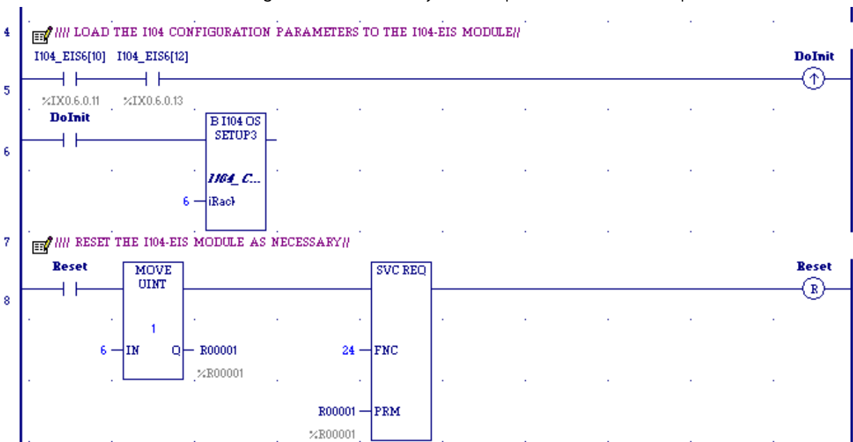
Figure 14: Ladder Logic Used to Configure IEC 104 Server Parameters
