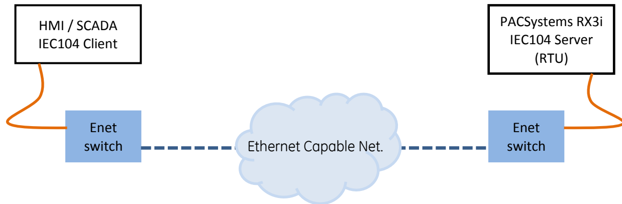
Figure 1: IEC 104 Basic System Architecture
