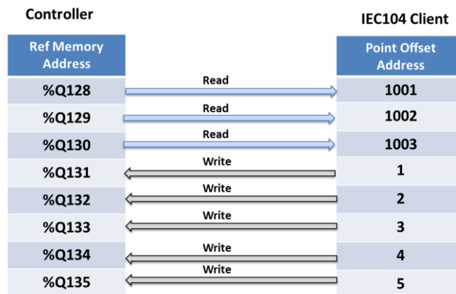
Figure 22: Read/Write Interaction between Controller and IEC104 Client (Case 4)
