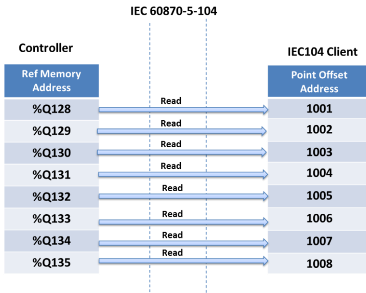
Figure 20: Red/Write Interaction between Controller and IEC104 Client (Case 3)
