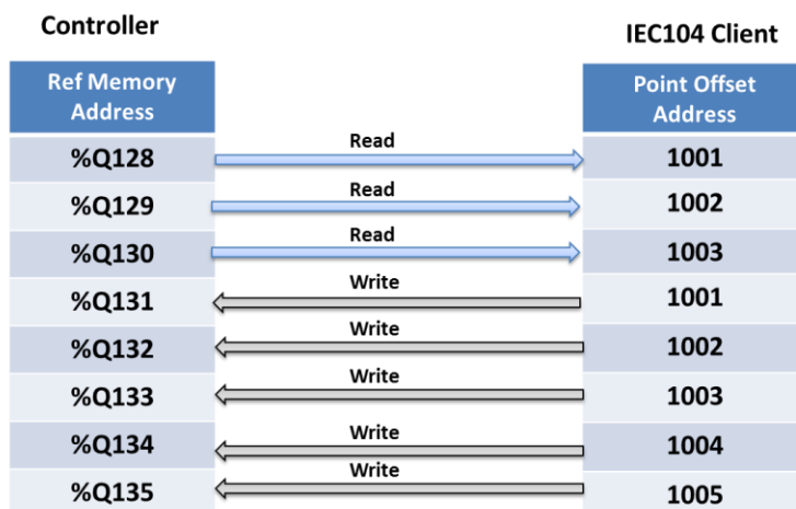
Figure 24: Red/Write Interaction between Controller and IEC104 Client (Case 5)
