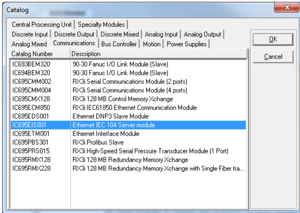
Figure 6: Selection of EIS001 for Installation
