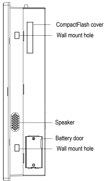
Figure 2.3 Side view of the panel PC
