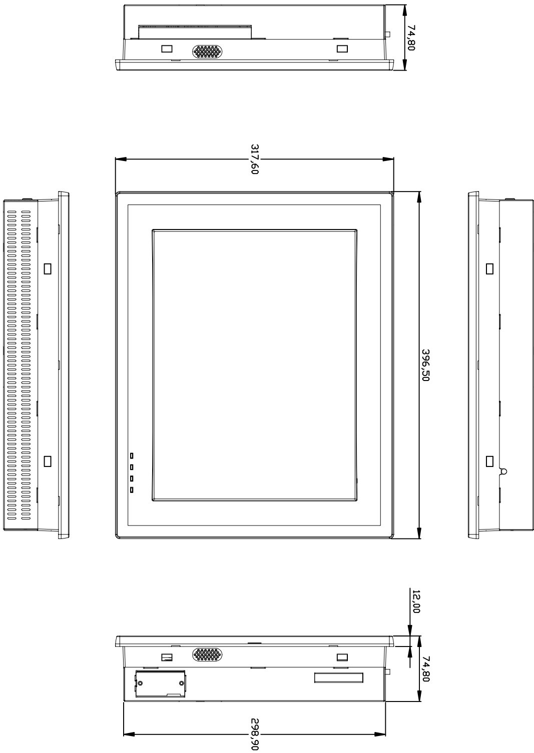
Figure 1.1 Dimensions of PPC-L157T
