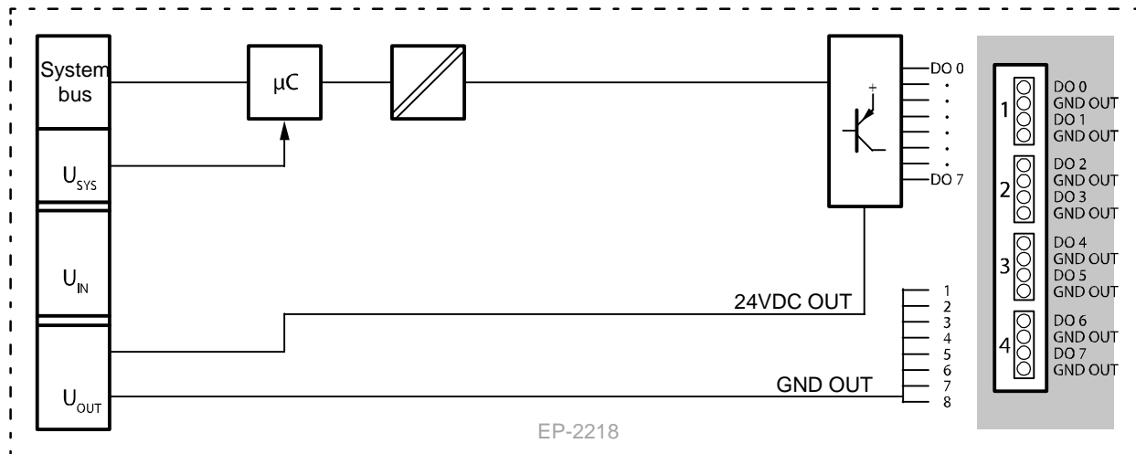
Block Diagram EP-2218
