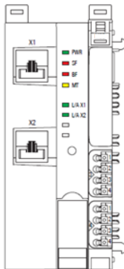
LED Status Indicators EPXMBE001
