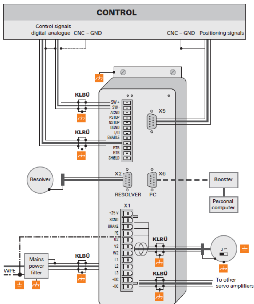
Connection Diagram of a Frequency Converter
