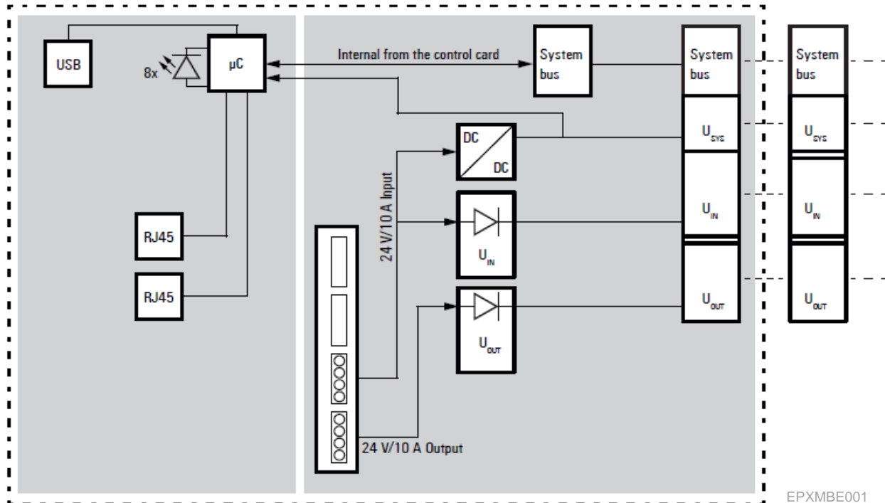
Block Diagram EPXMBE001
