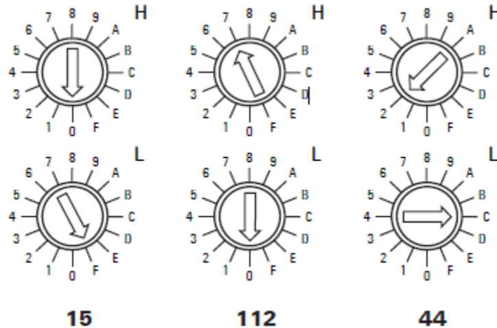
Examples for Addressing the EPXPBS001
