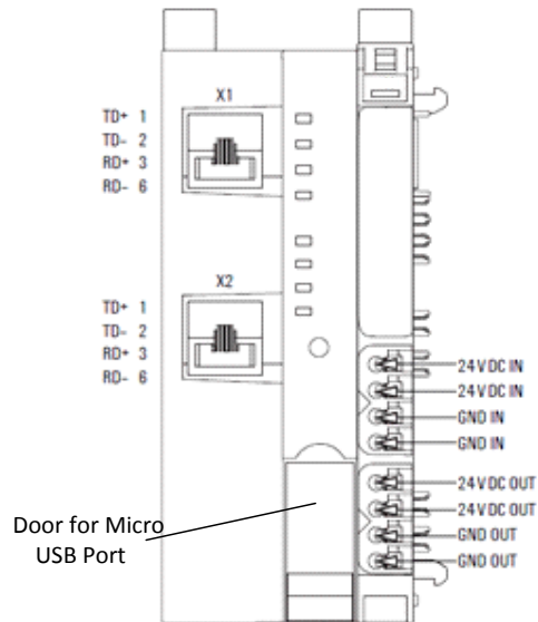
Connection Diagram EPXMBE001
