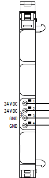
Connection Diagram EP-7631
