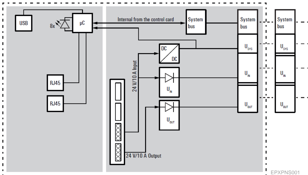
Block Diagram EPXPNS001
