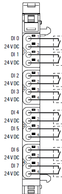
Connection Diagram EP-1218
