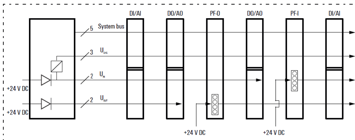
RSTi-EP Power Supply Concept
