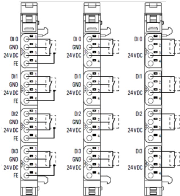
Connection Diagram EP-12F4
