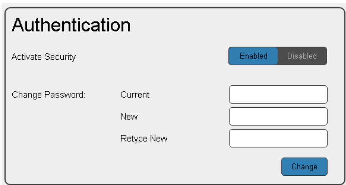
Figure 23: Authentication Page
