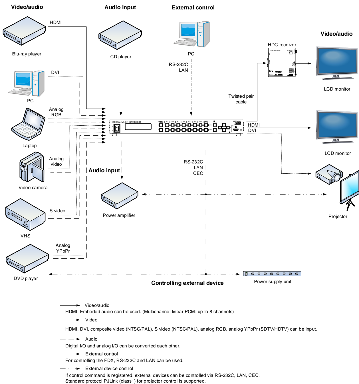
[Fig. 5.8] Source and sink devices are connected
