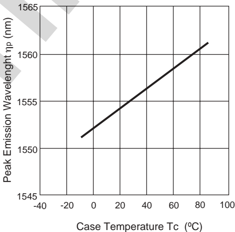
TEMPERATURE DEPENDENCE OF PEAK EMISSION WAVELENGTH
