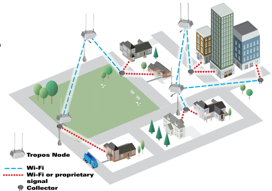
Tropos Metro-Scale Automated Utility Meter Reading Network
