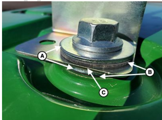
Right-Hand Cab Cap Screw Stackup
