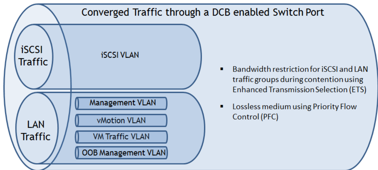
Figure 5: Conceptual View of Converged Traffic Using DCB
