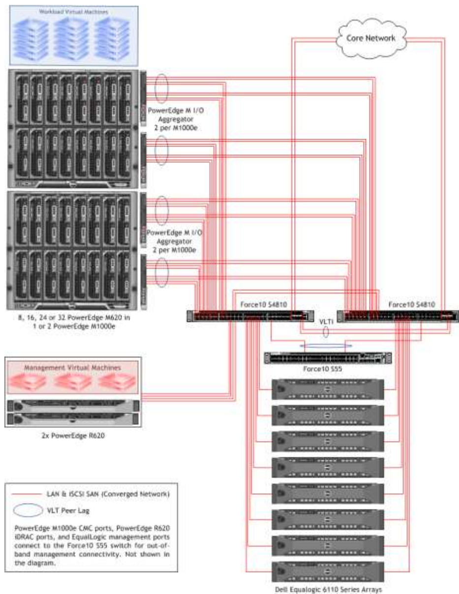
Figure 2: Active System 800v Network Topology (Logical View)
