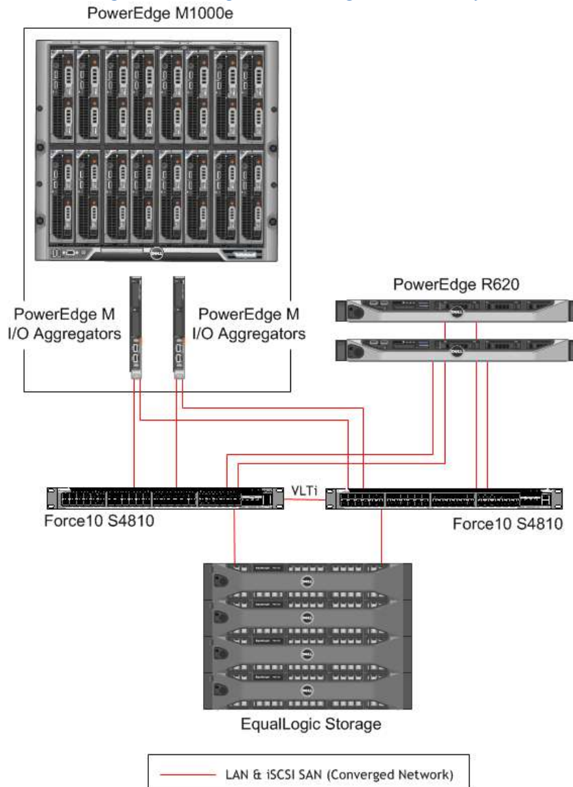
Figure 4: Converged Network Logical Connectivity
