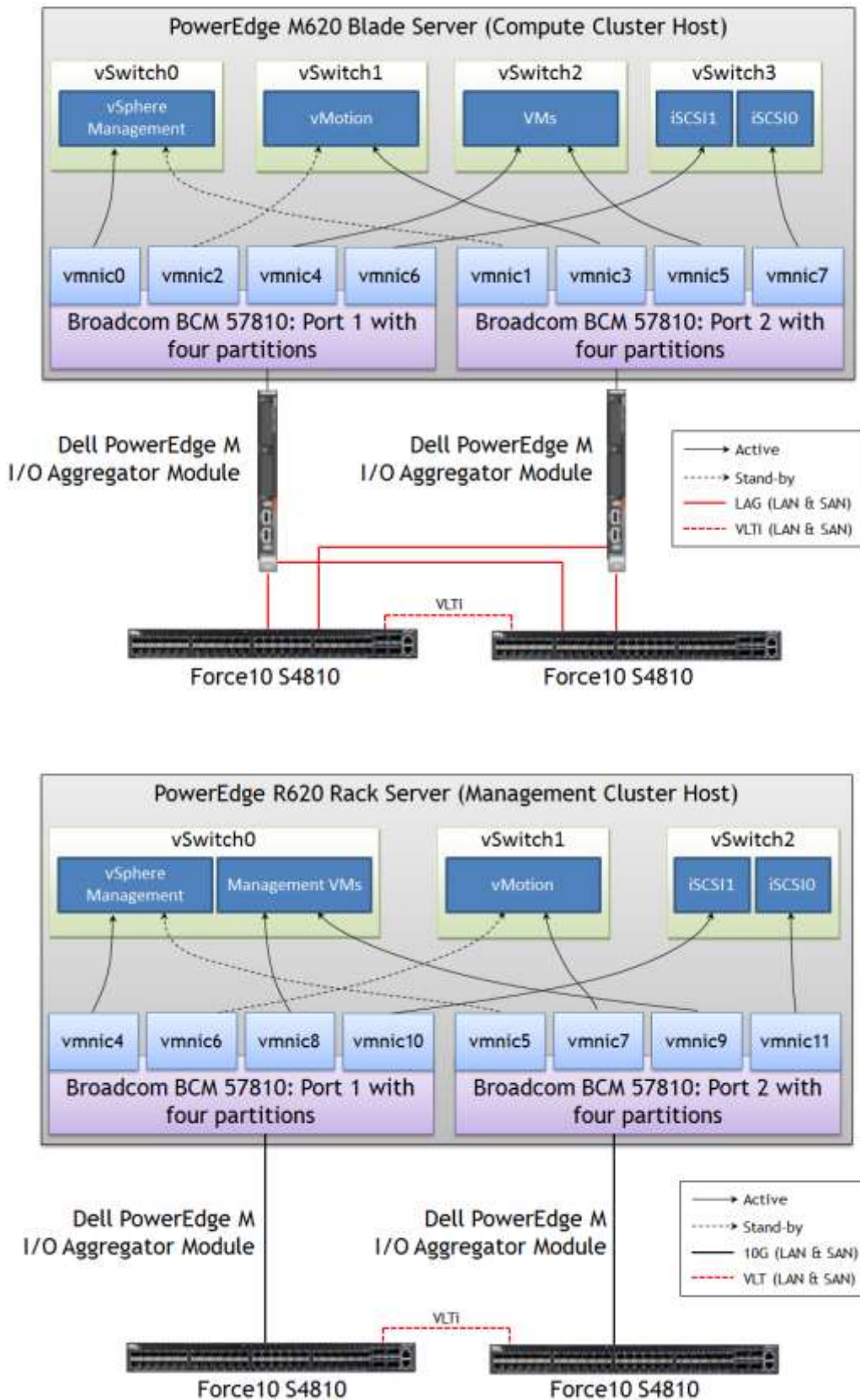
Figure 6: vSwitch and NPAR Configuration for the Hypervisor Hosts
