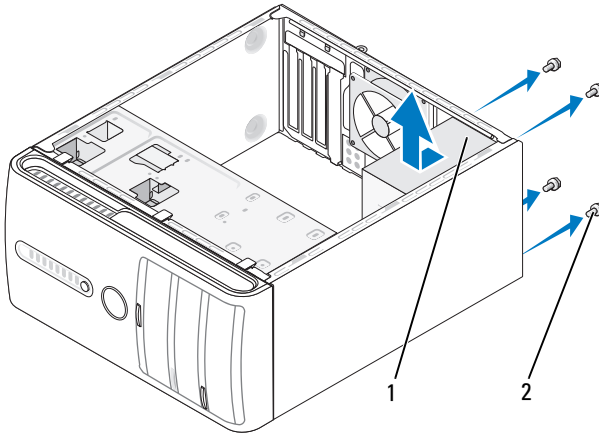
1 power supply 2 screws (4)
