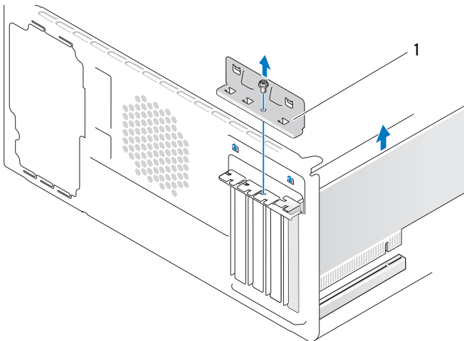
1 card retention bracket
