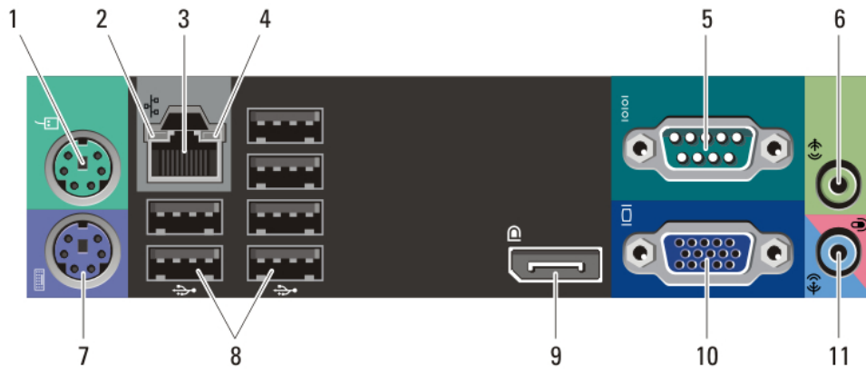
Figure 5. Back Panel View of Mini-Tower And Desktop
