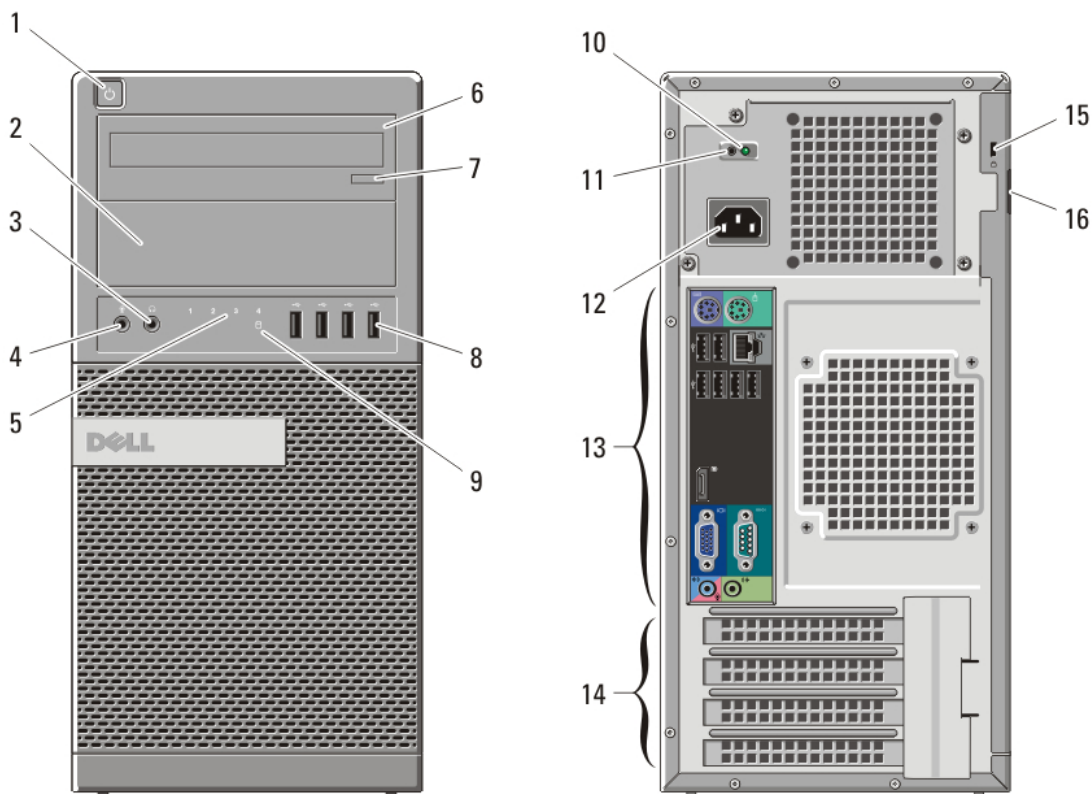
Figure 1. Front And Back View Of Mini-Tower
