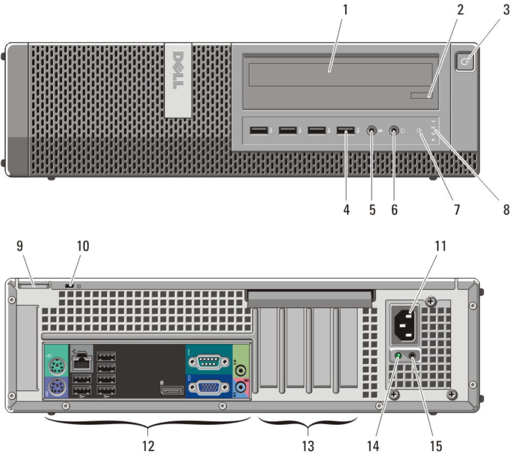
Figure 2. Front And Back View Of Desktop
