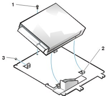
Figure 7. 3.5-Inch Diskette Drive Bracket
