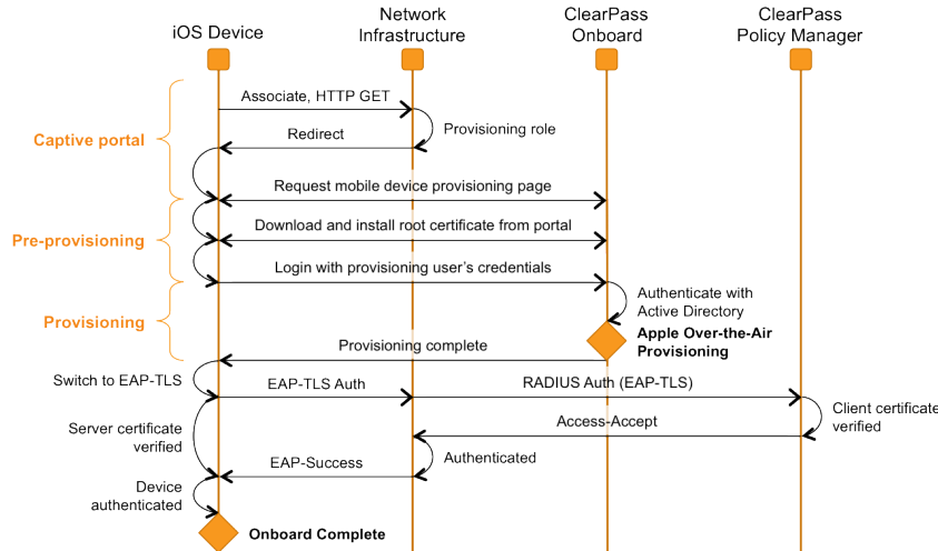
Figure 15 Sequence Diagram for the W-Onboard Workflow on iOS Platform
