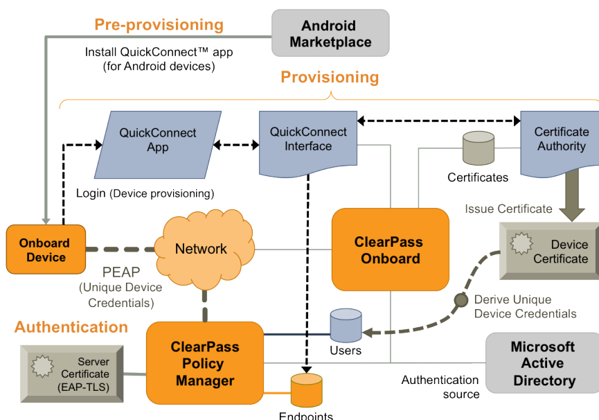
Figure 17 W-ClearPass Onboard Process for Onboard-Capable Devices
