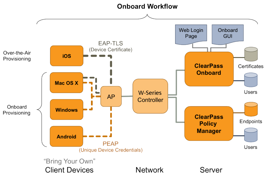
Figure 12 Detailed View of the W-ClearPass Onboard Network Architecture
