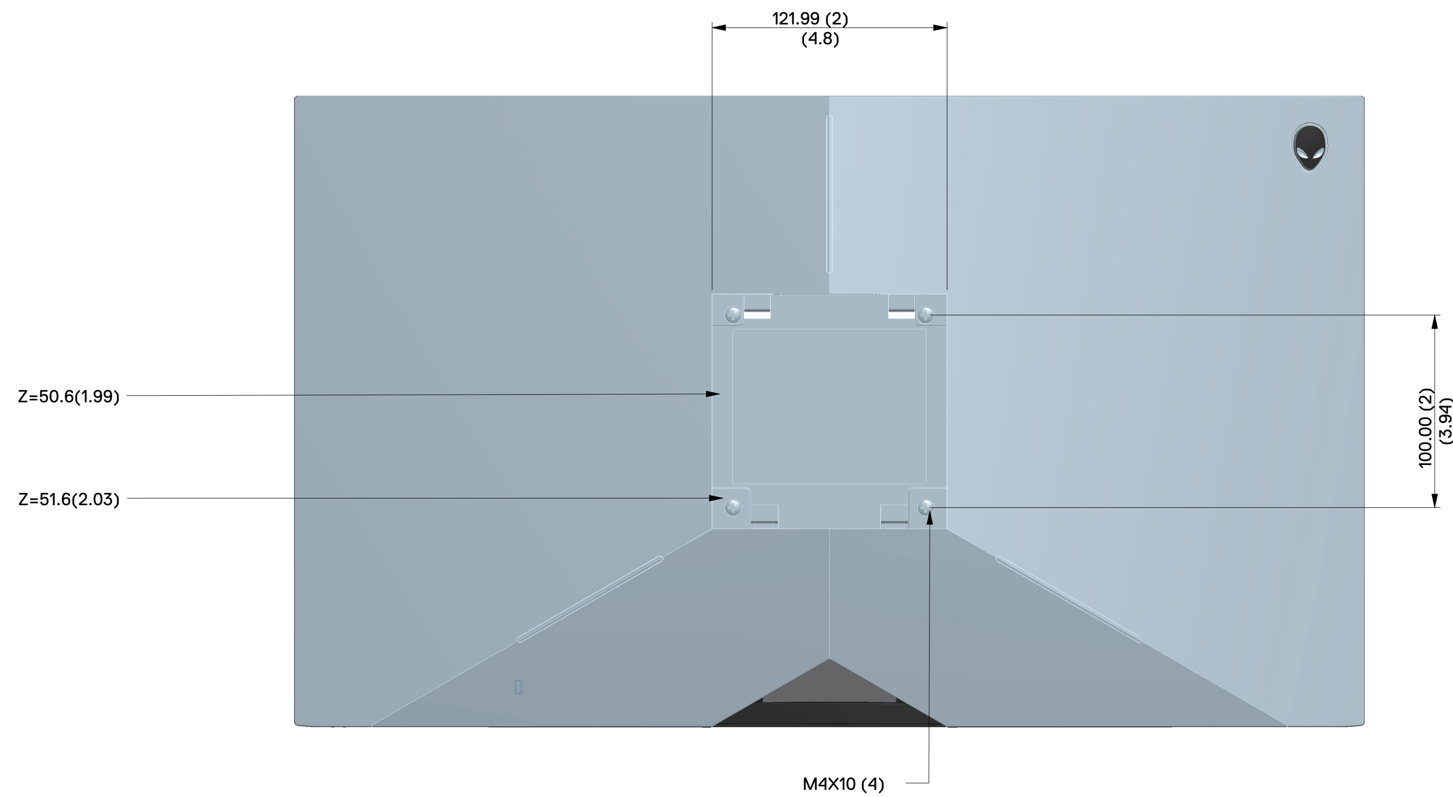
Back View of Monitor without stand
