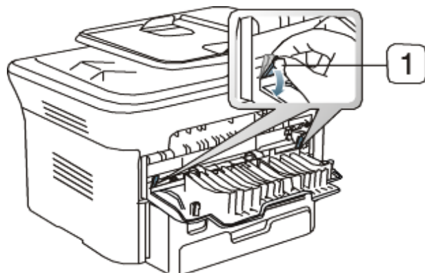
1. Pressure lever
