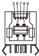
USB upstream port
