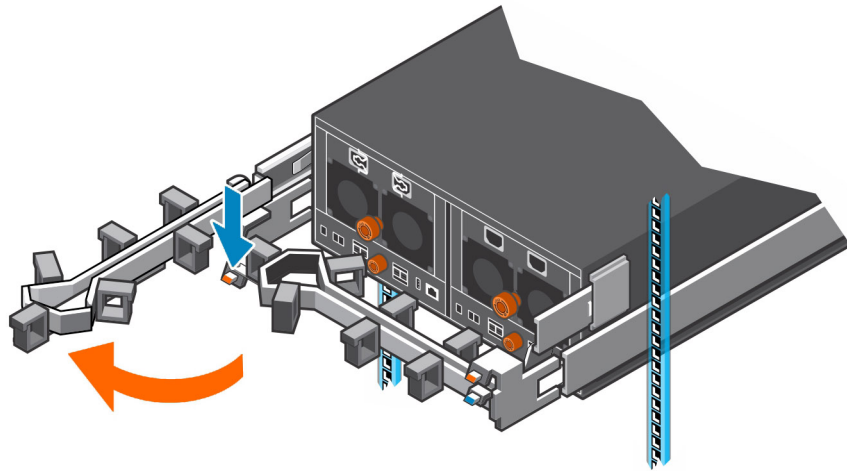
Figure 67. Pull Upper Arm Away from Chassis
