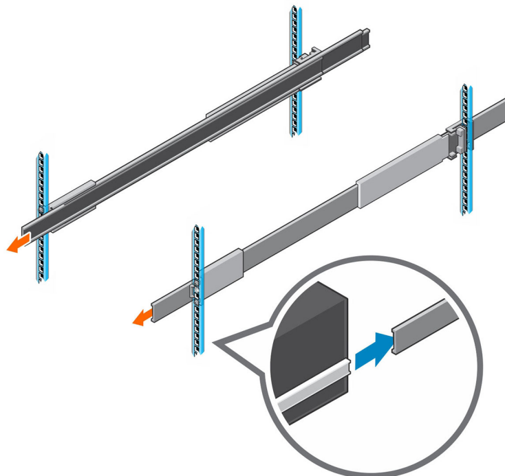
Figure 19. Extend the Rails from the Rack
