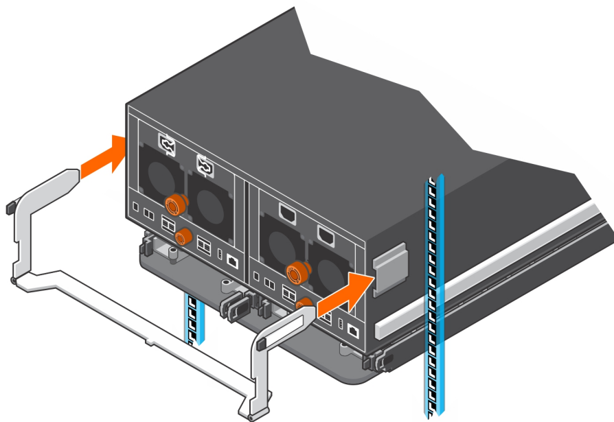
Figure 13. Install the Chassis Bracket to the Chassis
