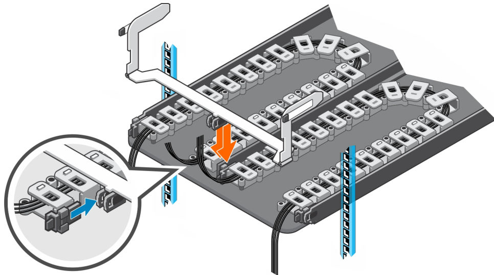
Figure 50. Disconnect Cable Chains from the Chassis Bracket
