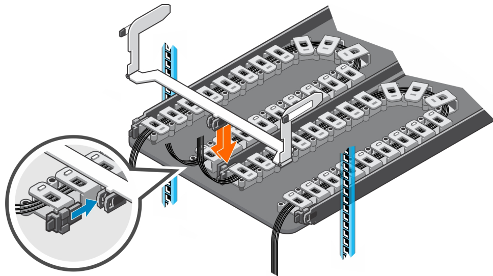
Figure 14. Clip Cable Chains to Chassis Bracket
