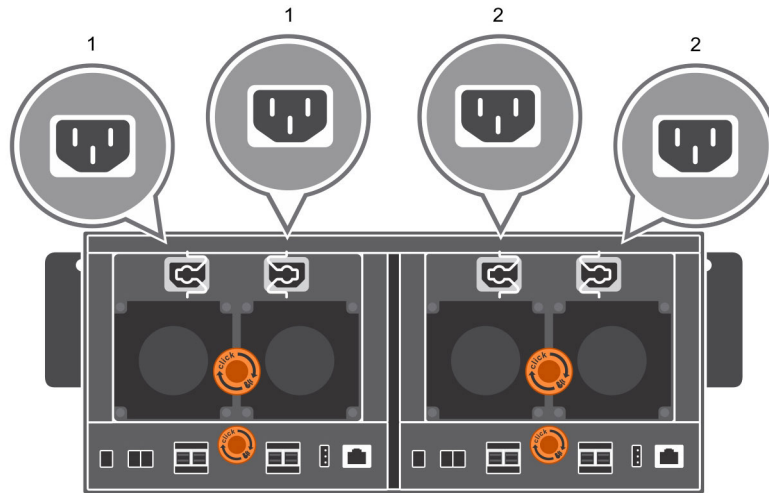
Figure 28. Connect Power Cables to the Power Supplies
