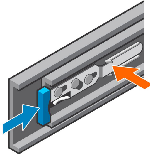
Figure 7. Push in Blue Tab on Expansion Enclosure Rails
