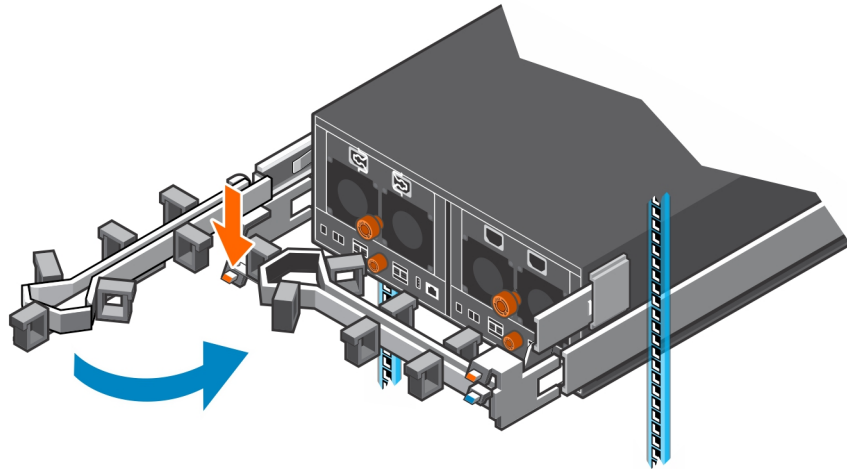
Figure 25. Swing Upper Arm to Right Side of Chassis and Secure Lower Arm
