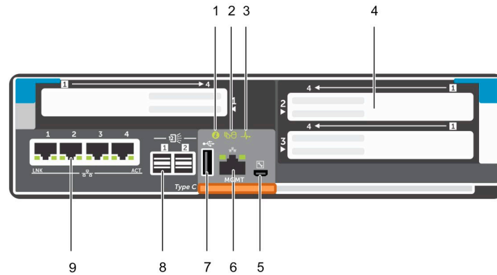
Figure 5. SC7020 Series Storage Controller
