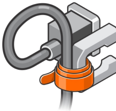
Figure 8. Removing the Hook and Loop Strap from the Power Cable
