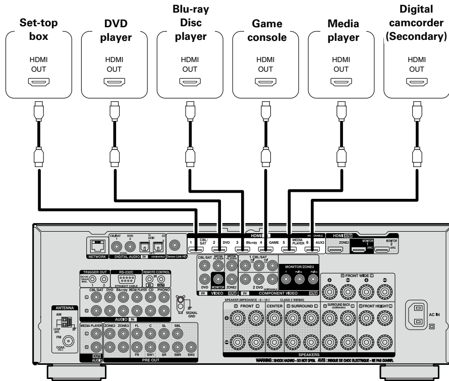
[Rear panel]
