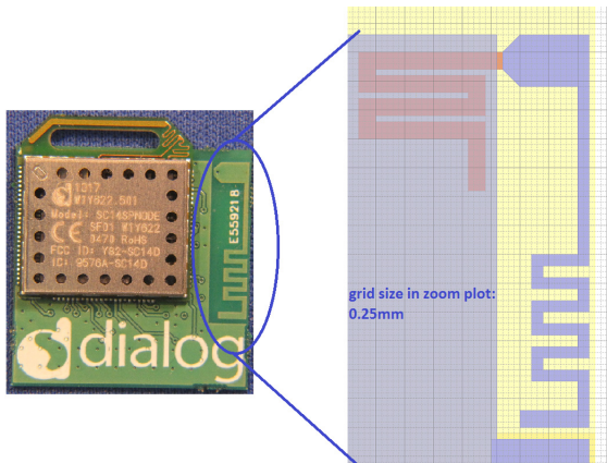
Figure 2 SC14CVMDECT_AF01_SF01 printed antenna design details
