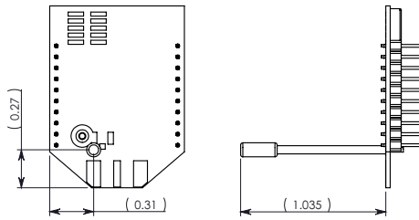
WIRE WHIP
