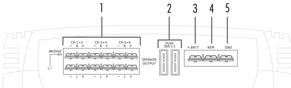
FIGURE 2—AMPLIFIER CONNECTIONS 6550 REAR
