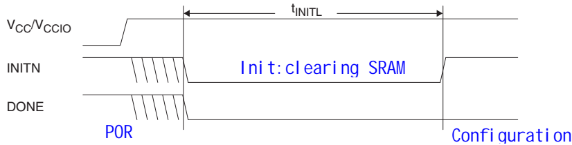
Figure 2. Configuration from Power-On-Reset Timing
