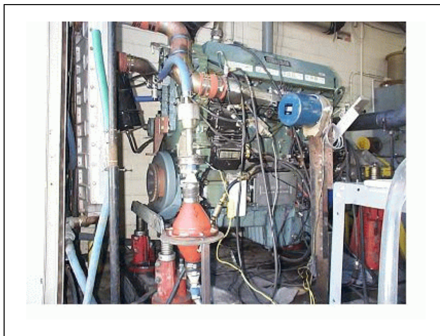
Figure 2. Baseline engine: a 1998 Detroit Diesel Corporation heavy-duty diesel engine, mounted in Southwest Research Institute's engine test cell #4.
